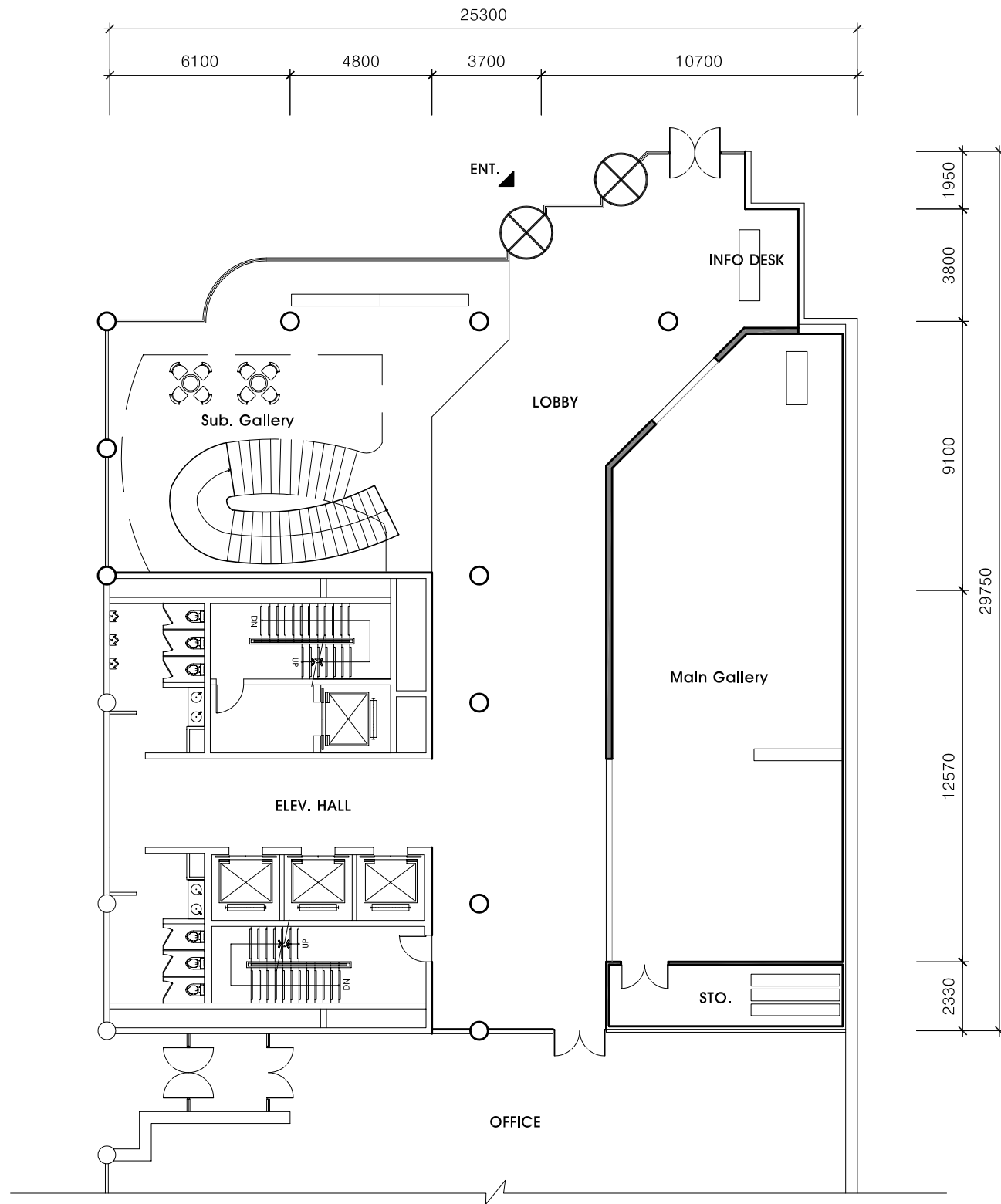
FLOOR PLAN
