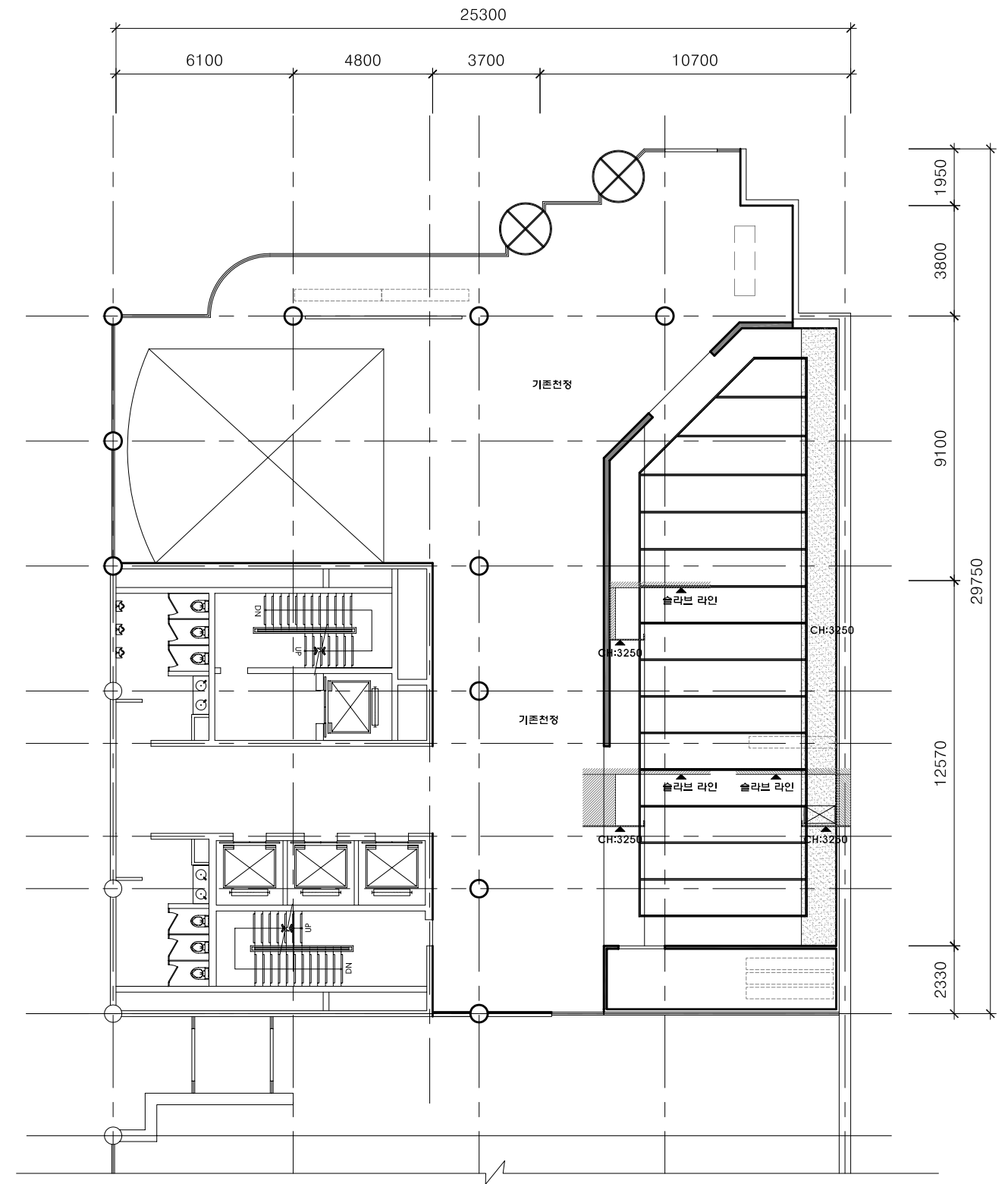
CEILING PLAN
